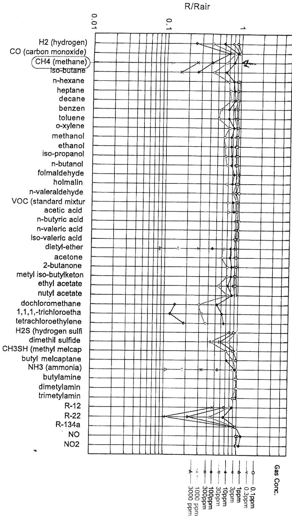
Fig 2b: SP-11 cross sensitivity data
